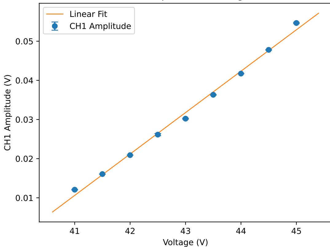
CH1 Amplitude vs Voltage
