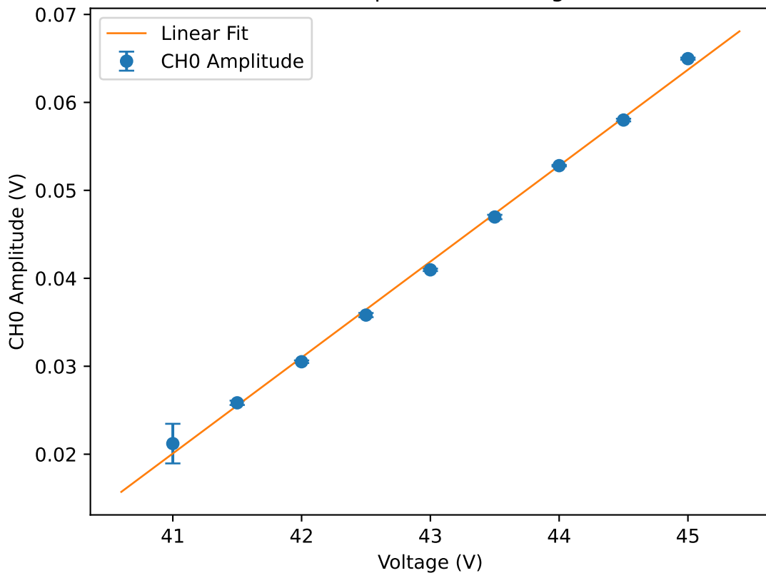
CH0 Amplitude vs Voltage
