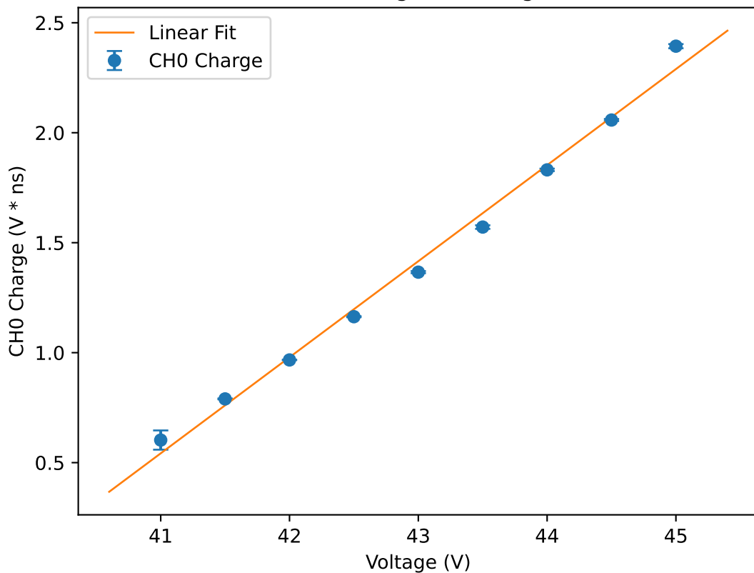
CH0 Charge vs Voltage
