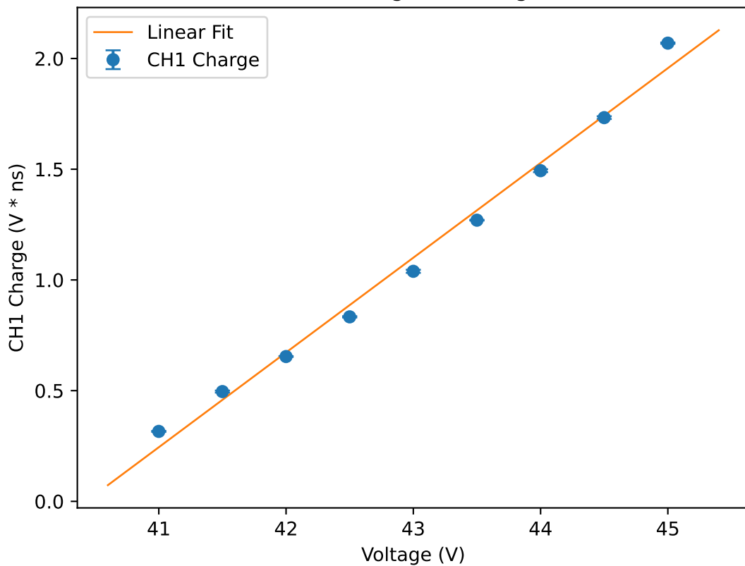
CH1 Charge vs Voltage
